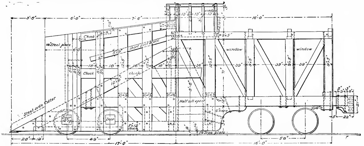
Fig. 408. Side Elevation of Framing.
